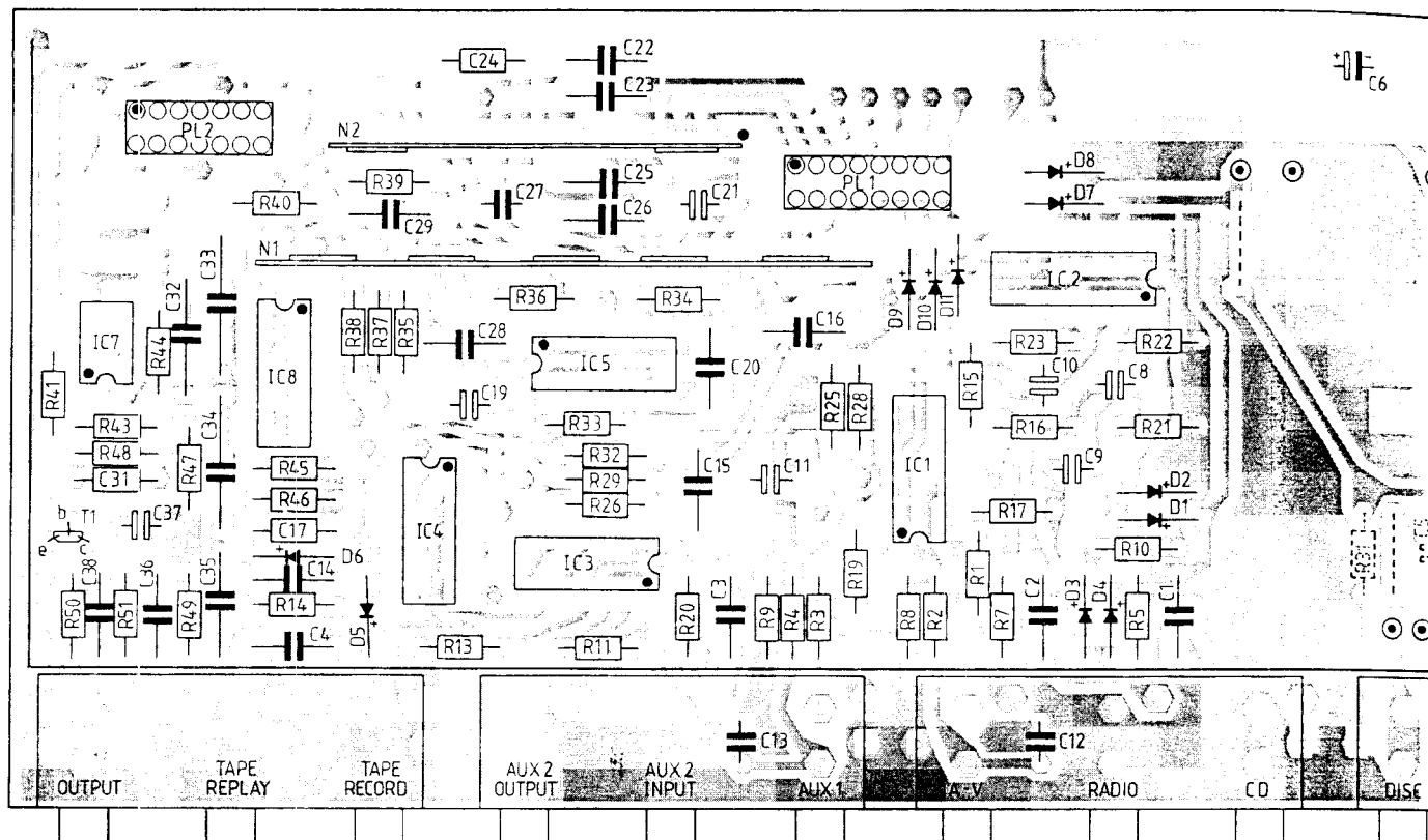
Audio PCB 2156-3-66
