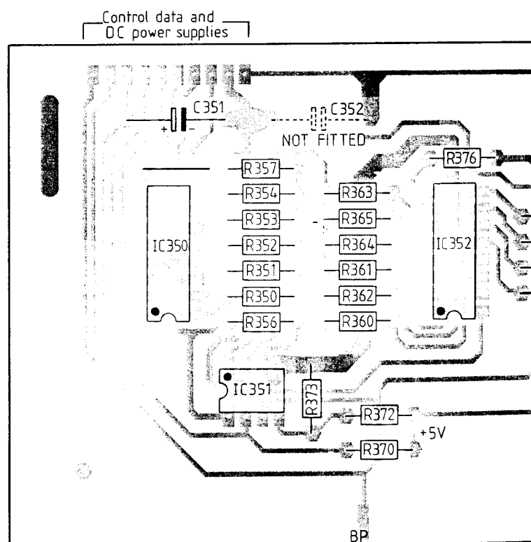
Top Display PCB 2196-5-66
