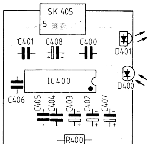
Receiver PCB 2181-6-66
