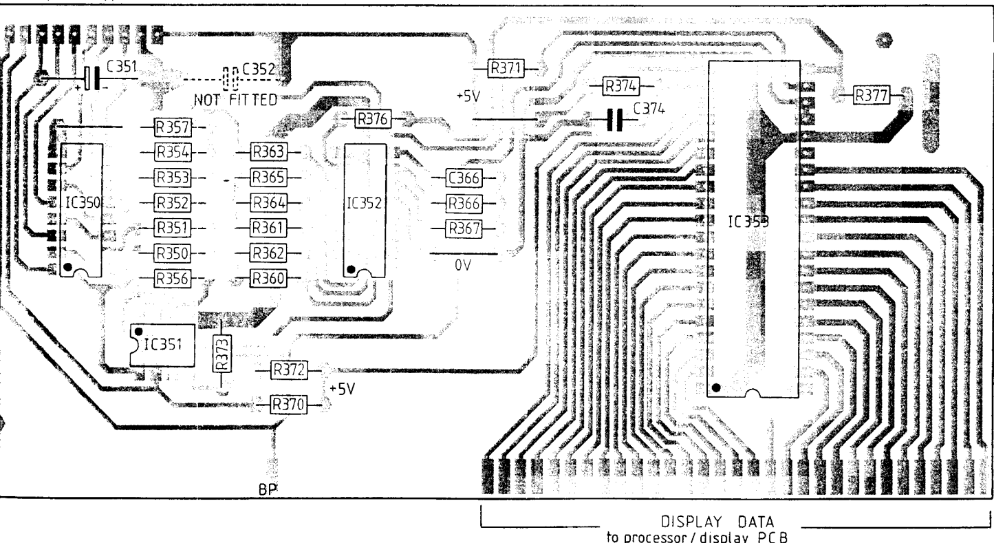
Display PCB 2196-5-66
