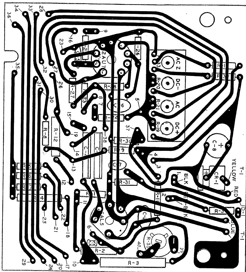
Figure 6. View of foil circuit of laminated board, showing components on opposite side
