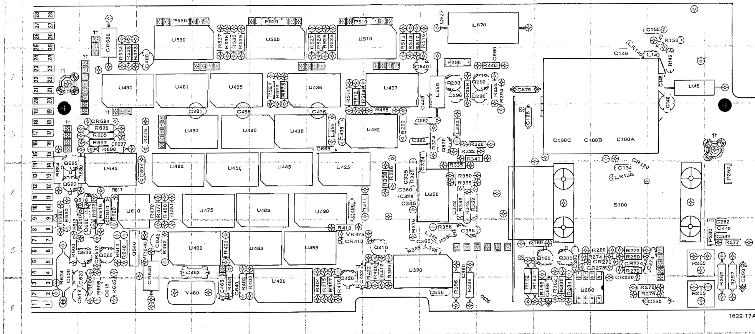
A1 Main circuit board "A" side.
